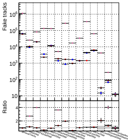
Number Symbol Label 1 ★ DOMstep3 TT ckrPixelLess 2 ✱ DOMstep3 TT default-relu4 3 ✱ DOMstep3 TT defaultNEWTOLDSAMPLE-relu4
