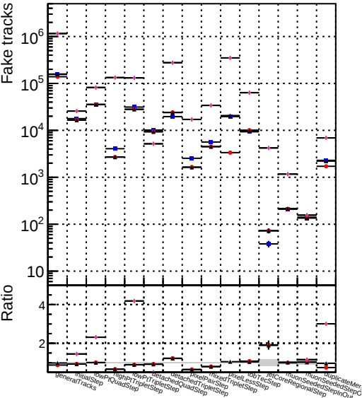
Number Symbol Variable 1 Black triangle DOMstep3 TT CKIPixelLess 2 Orange diamond DOMstep3 TT default-rlf4 3 Pink star DOMstep3 TT defaultNEWTOLDSAMPLE-rlf4
