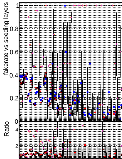
Fake rate vs. DOMestep3 DOMestep3+GKF DOMestep3+GKF+PileupLess
