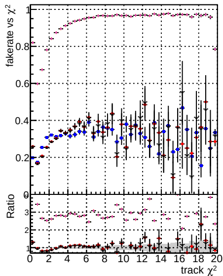
Fake rate vs. DOMestep3 DOMestep3+GKF DOMestep3+GKF+PileupLess
