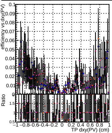
Efficiency vs Dxy(PV) DOMstep3 TT CKF DOMstep3 TT default DOMstep3 TT ckfPixelLess DOMstep3 TT default-relf3 DOMstep3 TT defaultNEWTOLDSAMPLE-relf3
