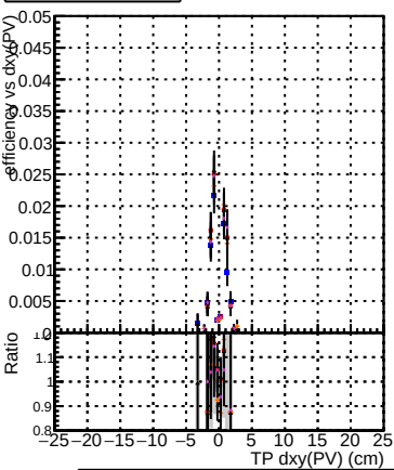
Efficiency vs Dxy(PV) DOMstep3 TT CKF DOMstep3 TT default DOMstep3 TT ckfPixelLess DOMstep3 TT default-relf3 DOMstep3 TT defaultNEWTOLDSAMPLE-relf3
