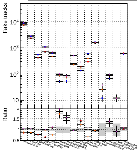
Number Series Configuration 1 Blue dot DOMstep3 TT CKF 2 Red dot DOMstep3 TT default 3 Black star DOMstep3 TT ckfPixelLess 4 Orange star DOMstep3 TT default-rlf3 5 Purple star DOMstep3 TT defaultNEWTOLDSAMPLE-rlf3
