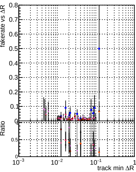
Fake rate vs ΔR(track, jet) for various models: DOM, Moten3, TT, GKE, default, etc. (NEWTOLD, SAMPLE-relf3)
