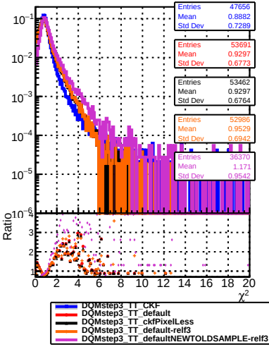
normalized \chi^2
