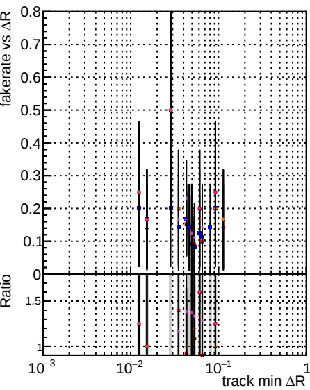
Fake rate vs \Delta R(\text{track, jet}) for DOM, Meten3, TT, GKE, CKKW, CKKWLLS, default, NEWTOLD, SAMPLE-reif3
