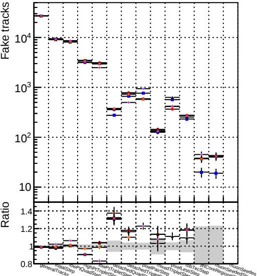
Number Symbol Label ▲ DOMstep3 TT ckrPixelLess ★ DOMstep3 TT default-relu3 ◆ DOMstep3 TT defaultNEWTOLDSAMPLE-relu3
