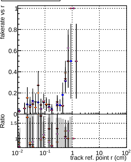
Fake rate vs v... DOM Meten3 GKF ... NEWTOLDSAMPLE-ref3
