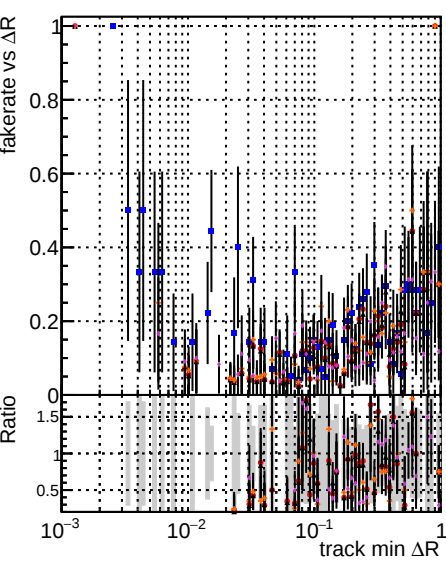
Fake rate vs \Delta R(\text{track, jet}) Duplicates Rate vs \Delta R(\text{track, jet}) Pileup rate vs \Delta R(\text{track, jet}) DOM Meten3 TT GKE default cell-less NEW TOLDSAMPLE-reif3
