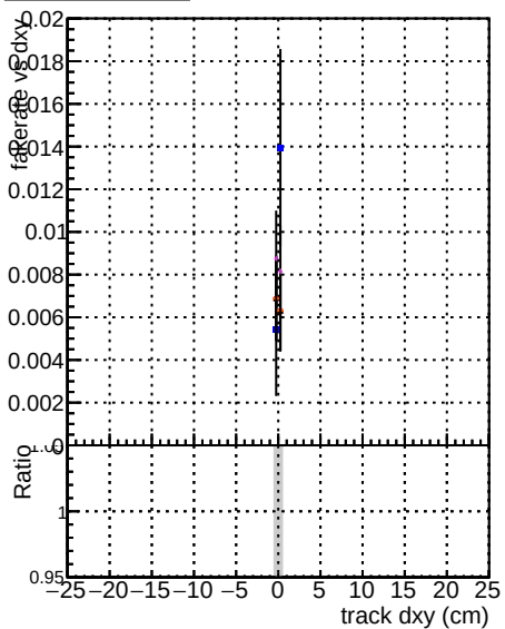
Method Fake rate DGM step 3 ~0.8 TT GKE ~0.6 TT default ~0.4 TT default less ~0.3 TT default NEW ~0.2
