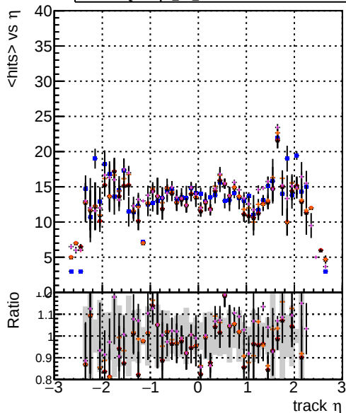
mean hits vs \eta DOMstep3 TT CKF DOMstep3 TT default DOMstep3 TT ckPixelLess DOMstep3 TT default-relf3 DOMstep3 TT default-NEWTOLDSAMPLE-relf3
