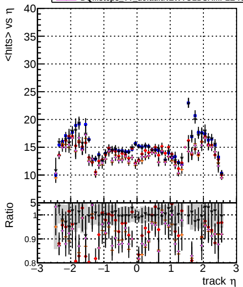
mean hit DOMstep3 TT CKF DOMstep3 TT default DOMstep3 TT ckPixelLess DOMstep3 TT default-relf3 DOMstep3 TT defaultNEWTOLDSAMPLE-relf3
