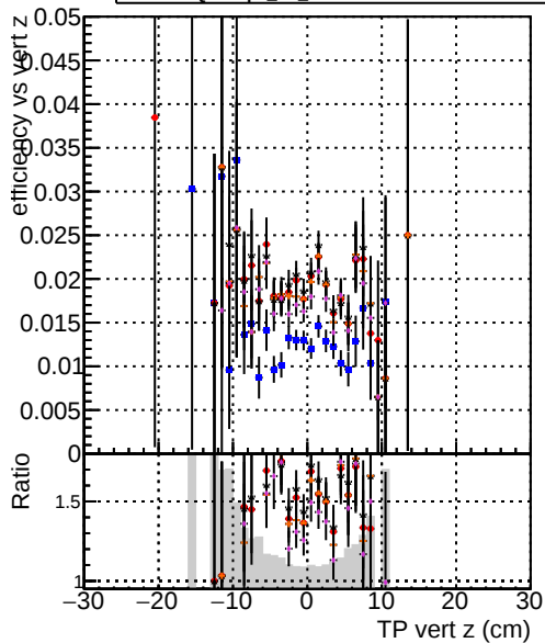
Efficiency Series Configuration ~0.85 DOMstep3 TT cktPixelLess ~0.75 DOMstep3 TT default-relf3 ~0.65 DOMstep3 TT defaultNEWTOLDSAMPLE-relf3
