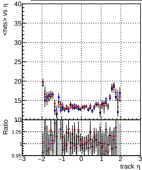
mean hit DOMstep3 TT CKF DOMstep3 TT default DOMstep3 TT ckrPixelLess DOMstep3 TT default-relf3 DOMstep3 TT defaultNEWTOLDSAMPLE-relf3
