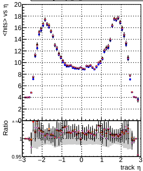
mean hit DOMstep3 TT CKF DOMstep3 TT ckfPixelLess DOMstep3 TT default-relf3 DOMstep3 TT default-NEWTOLDSAMPLE-relf3
