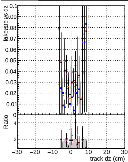
Model Fake rate DOMstep3 ~0.15 TT GKE default ~0.25 TT GKE full ~0.15 TT GKE less ~0.05 TT default ~0.35
