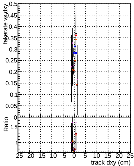
Model Fake rate vs d DOMstep3 ~0.1 TT ~0.2 GKE ~0.3 default ~0.4 less ~0.5 NEW ~0.6
