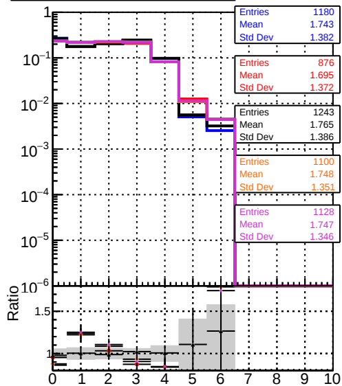
mean hit DOMstep3 CKF DOMstep3 default DOMstep3 ckfPixelLess DOMstep3 default-relf3 DOMstep3 defaultNEWTOLDSAMPLE-relf3
