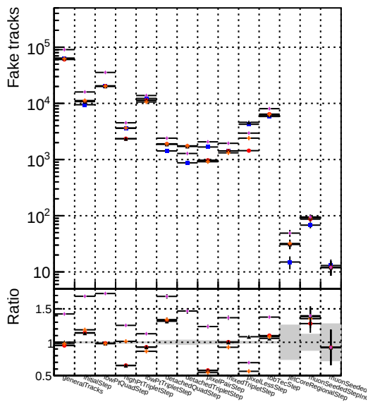
Number Symbol Label 1 Black triangle DOMstep3 TT cklPixelLess 2 Orange cross DOMstep3 TT default-rlf3 3 Purple asterisk DOMstep3 TT defaultNEWTOLDSAMPLE-rlf3
