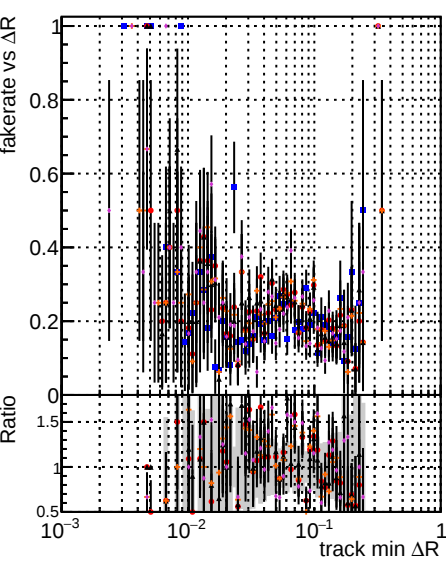
Fake rate vs \Delta R(\text{track, jet}) Duplicates rate vs \Delta R(\text{track, jet}) Pileup rate vs \Delta R(\text{track, jet}) DOM Meten3 TT GKE default NewTOLDSAMPLE-reif3
