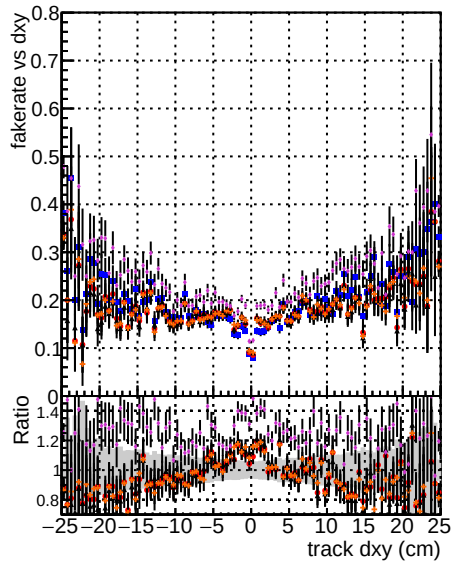
Fake rate vs d Duplicates rate vs dxy Pileup rate vs dxy Ratio track dxy (cm)
