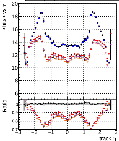
mean hits vs \eta DOMstep3 TT CKF DOMstep3 TT ckPixelLess DOMstep3 TT default-relf3 DOMstep3 TT default-NEWTOLDSAMPLE-relf3
