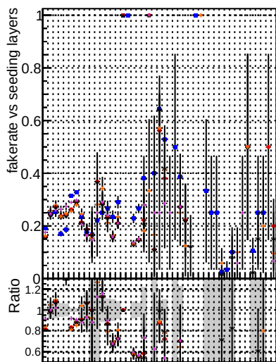
Fake rate vs. DOMstep3 DOMstep3TT GK5 default GK5Less defaultLess NEWT
