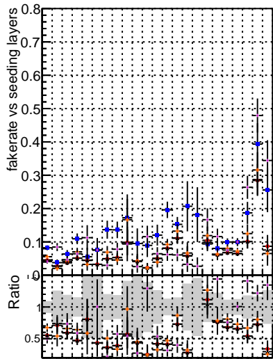
Fake rate vs. DQMstop3 CKE CKE+Pileless CKE+Pileless+OLD CKE+Pileless+OLD+SAMPLE-ref2 NEW
