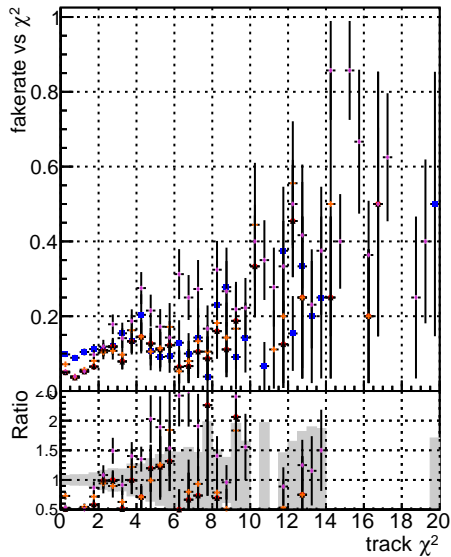
Fake rate vs. DQMstop3 CKE CKE+Pileless CKE+Pileless+OLD CKE+Pileless+OLD+SAMPLE-ref2 NEW
