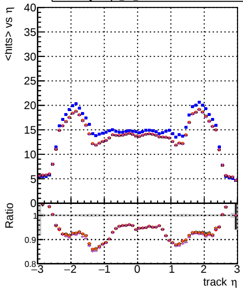
mean hit DOMstep3 TT CKF DOMstep3 TT default DOMstep3 TT ckPixelLess DOMstep3 TT default-relf2 DOMstep3 TT defaultNEWTOLDSAMPLE-relf2
