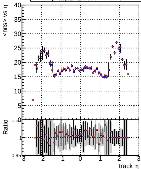
mean hit DOMstep3 TT CKF DOMstep3 TT default DOMstep3 TT ckrPixelLess DOMstep3 TT default-relf2 DOMstep3 TT defaultNEWTOLDSAMPLE-relf2
