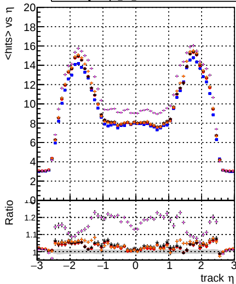
DOMstep3 TT CKF DOMstep3 TT default DOMstep3 TT ckPixelLess DOMstep3 TT default-relf2 DOMstep3 TT defaultNEWTOLDSAMPLE-relf2 mean hits
