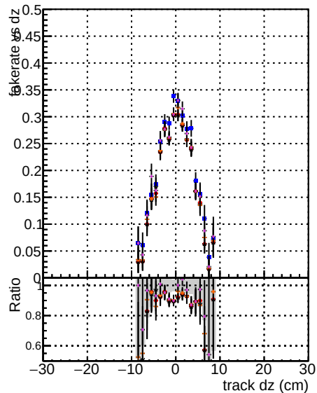
Fake rate vs dz DOMstep3+GKF+Pileless DOMstep3+GKF+Pileless+OLDSAMPLE+relf2
