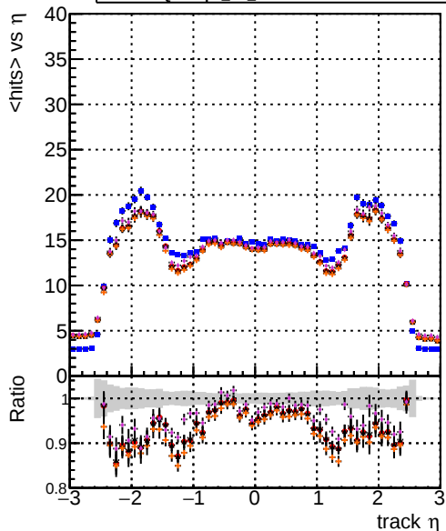
DOMstep3 TT CKF DOMstep3 TT ckPixelLess DOMstep3 TT default-rlf2 DOMstep3 TT defaultNEWTOLDSAMPLE-rlf2 mean hit
