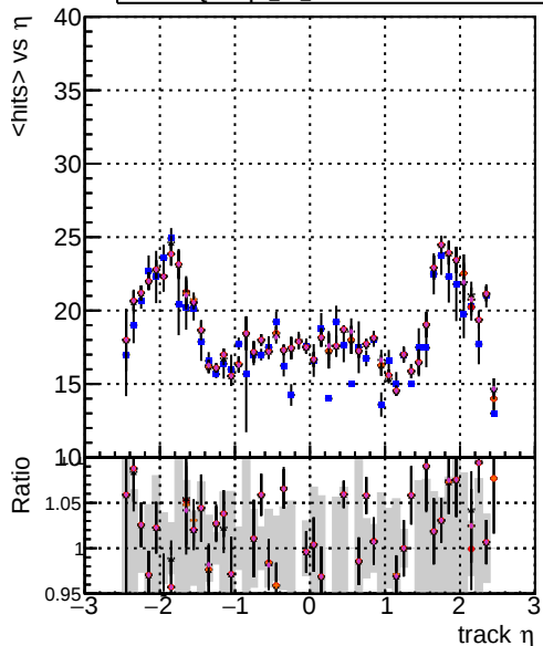
mean hit DOMstep3 CKF default DOMstep3 CKFPixelLess DOMstep3 default-relf2 DOMstep3 defaultNEWTOLDSAMPLE-relf2
