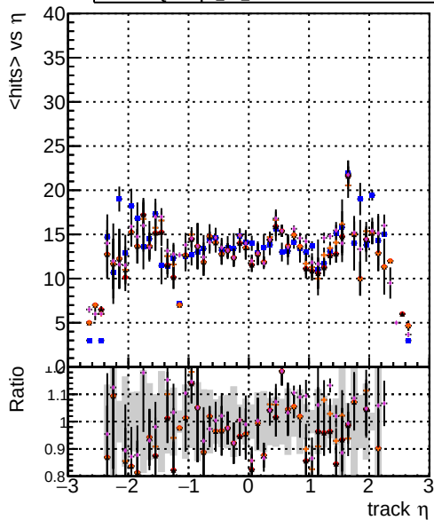
mean hits vs \eta DOMstep3 CKF DOMstep3 default DOMstep3 ckrPixelLess DOMstep3 default-relf2 DOMstep3 default-NEWTOLDSAMPLE-relf2
