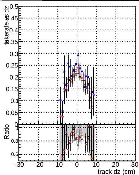
Fake rate vs dz DOMstep3+GKF+Pileupless+OLD+NEW+TDSAMPLE+relf2
