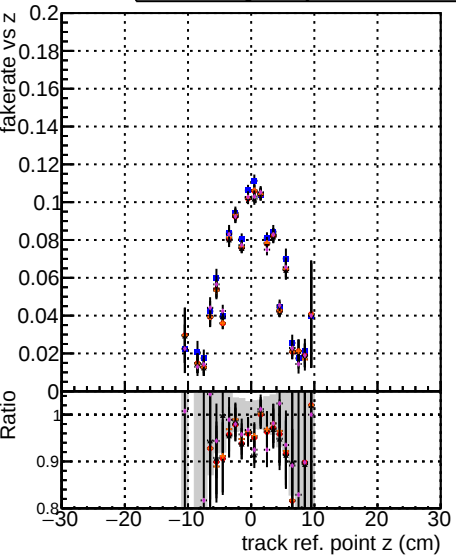
Fake rate vs v NEWTOLDSAMPLE-ref2
