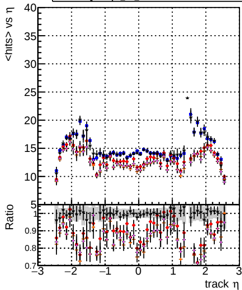
DOMstep3 TT CKF DOMstep3 TT default DOMstep3 TT ckfPixelLess DOMstep3 TT default-relf2 DOMstep3 TT defaultNEWTOLDSAMPLE-relf2 mean hit
