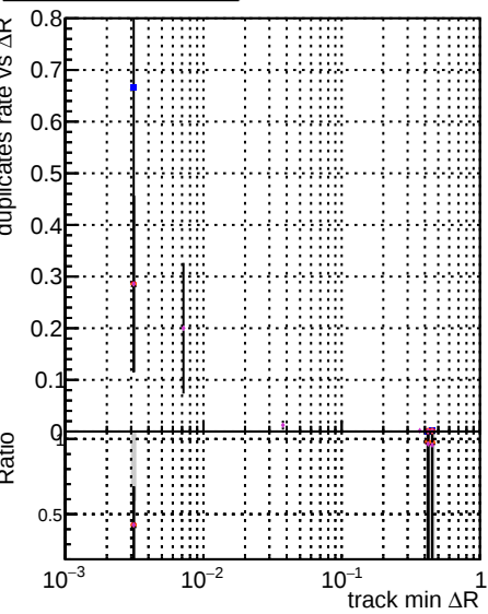
Fake rate vs \Delta R(\text{track, jet}) Duplicates rate vs \Delta R(\text{track, jet}) Pileup rate vs \Delta R(\text{track, jet}) DOM Meten3 TT GKE default CKP CKP+less NEWTOLD SAMPLE-relf2
