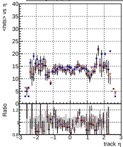
mean hit DOMstep3 CKF DOMstep3 default DOMstep3 ckrPixelLess DOMstep3 default-relf2 DOMstep3 defaultNEWTOLDSAMPLE-relf2
