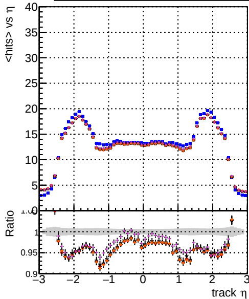
mean hit DOMstep3 TT CKF DOMstep3 TT default DOMstep3 TT ckfPixelLess DOMstep3 TT default-relf2 DOMstep3 TT defaultNEWTOLDSAMPLE-relf2
