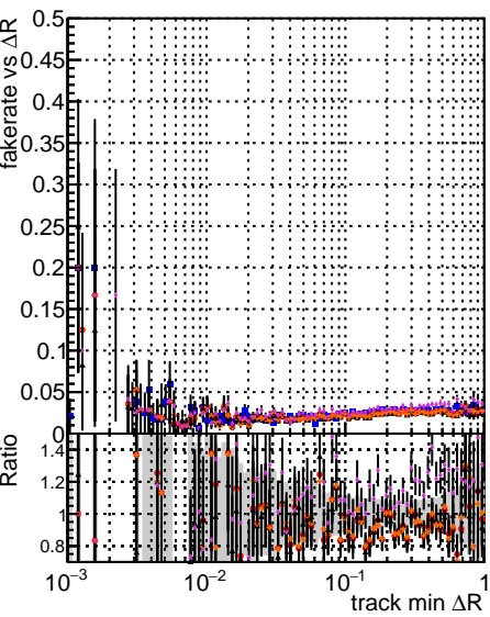
Fake rate vs \Delta R(\text{track, jet}) Duplicates rate vs \Delta R(\text{track, jet}) Pileup rate vs \Delta R(\text{track, jet}) Legend: DOM, GKF, default, NEWTOLD, SAMPLE-ref2, etc.
