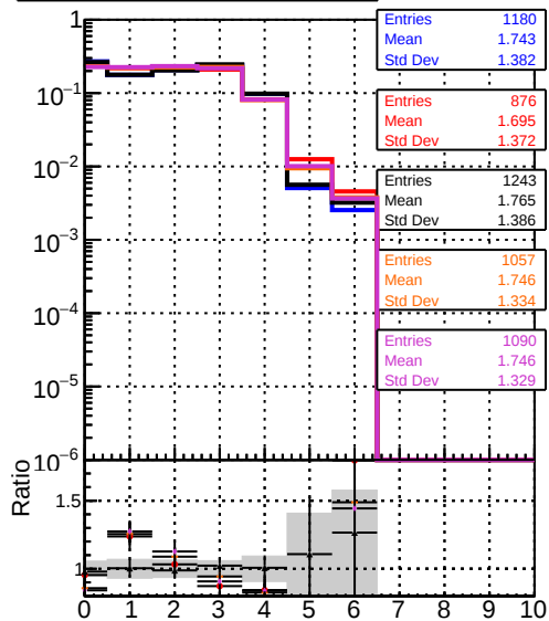
mean hit DOMstep3 TT CKF DOMstep3 TT default DOMstep3 TT ckfPixelLess DOMstep3 TT default-relf2 DOMstep3 TT defaultNEWTOLDSAMPLE-relf2
