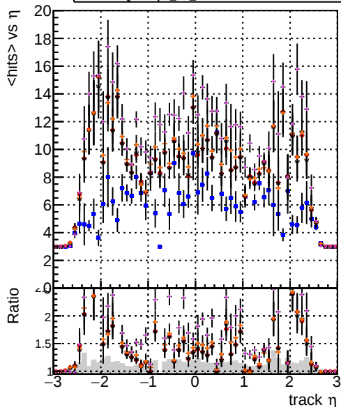
mean hit DOMstep3 TT CKF DOMstep3 TT default DOMstep3 TT ckPixelLess DOMstep3 TT default-relf2 DOMstep3 TT defaultNEWTOLDSAMPLE-relf2
