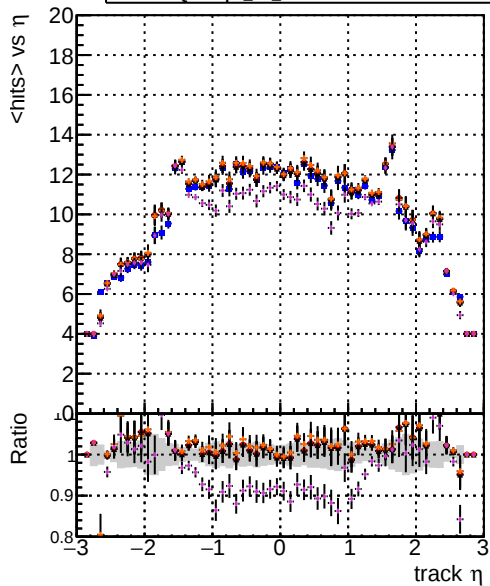
mean hits vs \eta DOMstep3 TT CKF DOMstep3 TT default DOMstep3 TT ckfPixelLess DOMstep3 TT default-relf2 DOMstep3 TT defaultNEWTOLDSAMPLE-relf2
