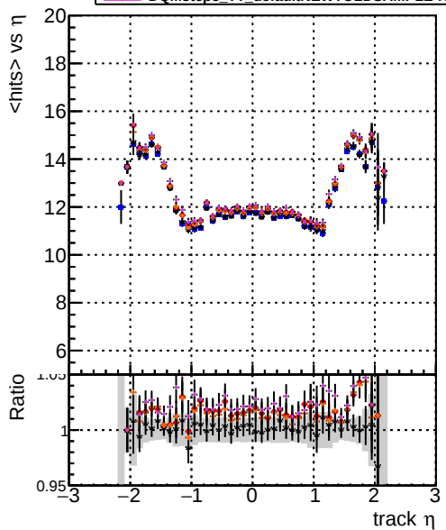
DOMstep3 CKF DOMstep3 default DOMstep3 ckPixelLess DOMstep3 default-rlf2 DOMstep3 defaultNEWTOLDSAMPLE-rlf2 mean hit
