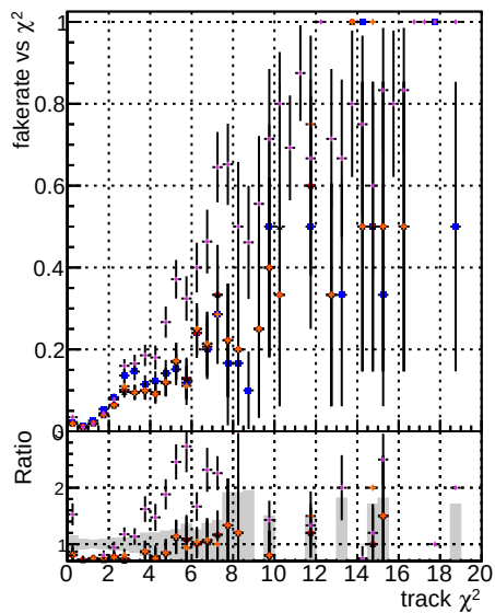
Fake rate vs. DOMestep3 DOMestep3+GKF DOMestep3+GKF+Pileupless Default NEWTOLD SAMPLE-relf2
