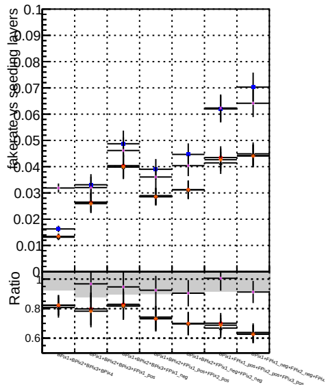
Fake rate vs. DOMestep3 DOMestep3+GKF DOMestep3+GKF+Pileupless Default NEWTOLD SAMPLE-relf2
