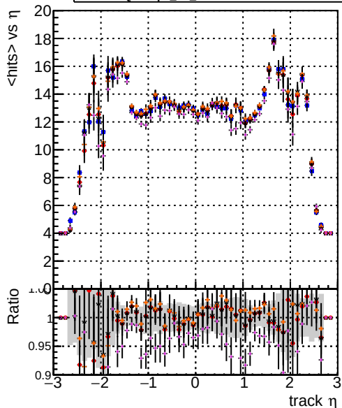
mean hits DOMstep3 TT CKF DOMstep3 TT default DOMstep3 TT ckfPixelLess DOMstep3 TT default-relf2 DOMstep3 TT defaultNEWTOLDSAMPLE-relf2
