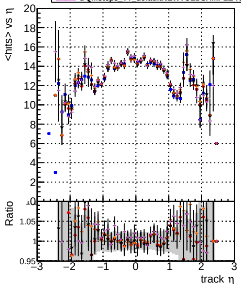
mean hits DOMstep3 TT CKF DOMstep3 TT default DOMstep3 TT ckfPixelLess DOMstep3 TT default-relf2 DOMstep3 TT defaultNEWTOLDSAMPLE-relf2
