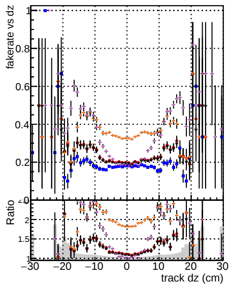
Model Fake rate DOMstep3 ~0.15 TT GKE default ~0.25 TT GKE full ~0.20 TT GKE less ~0.10 TT default ~0.30
