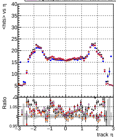
mean hits vs \eta DOMstep3 CKF DOMstep3 default DOMstep3 ckfPixelLess DOMstep3 default-relf2 DOMstep3 default-NEWTOLDSAMPLE-relf2
