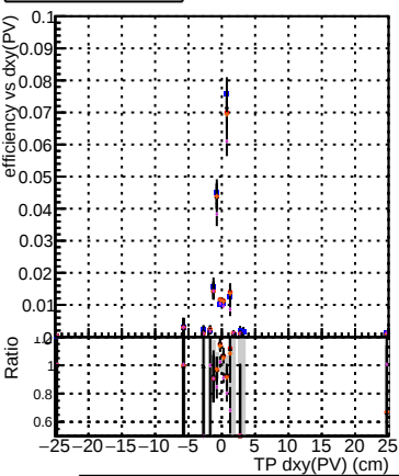
Efficiency vs Dxy(PV) DOMstep3 TT CKF DOMstep3 TT default DOMstep3 TT ckfPixelLess DOMstep3 TT default-relf DOMstep3 TT defaultNEWTOLDSAMPLE-relf
